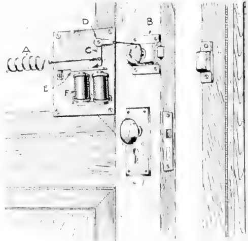
Essentials in the Arrangement for Unlocking Door Without a Key
